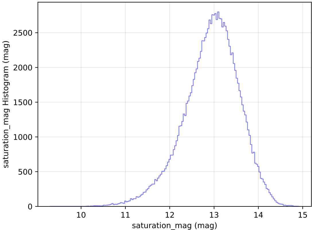
too_10_4v3.4_10yrs All sky u band: saturation_mag Histogram
