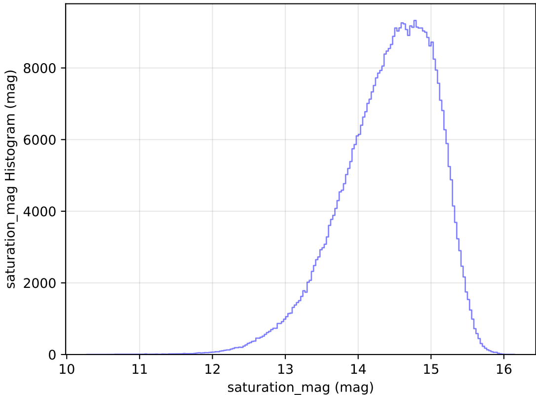
too_10_4v3.4_10yrs All sky i band: saturation_mag Histogram
