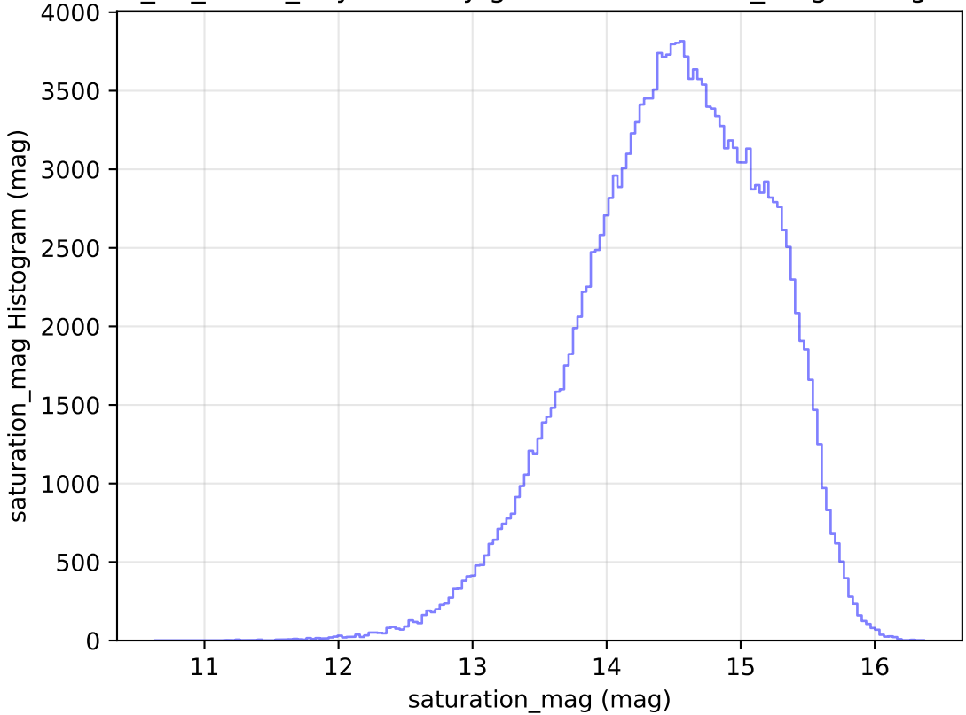
too_10_4v3.4_10yrs All sky g band: saturation_mag Histogram
