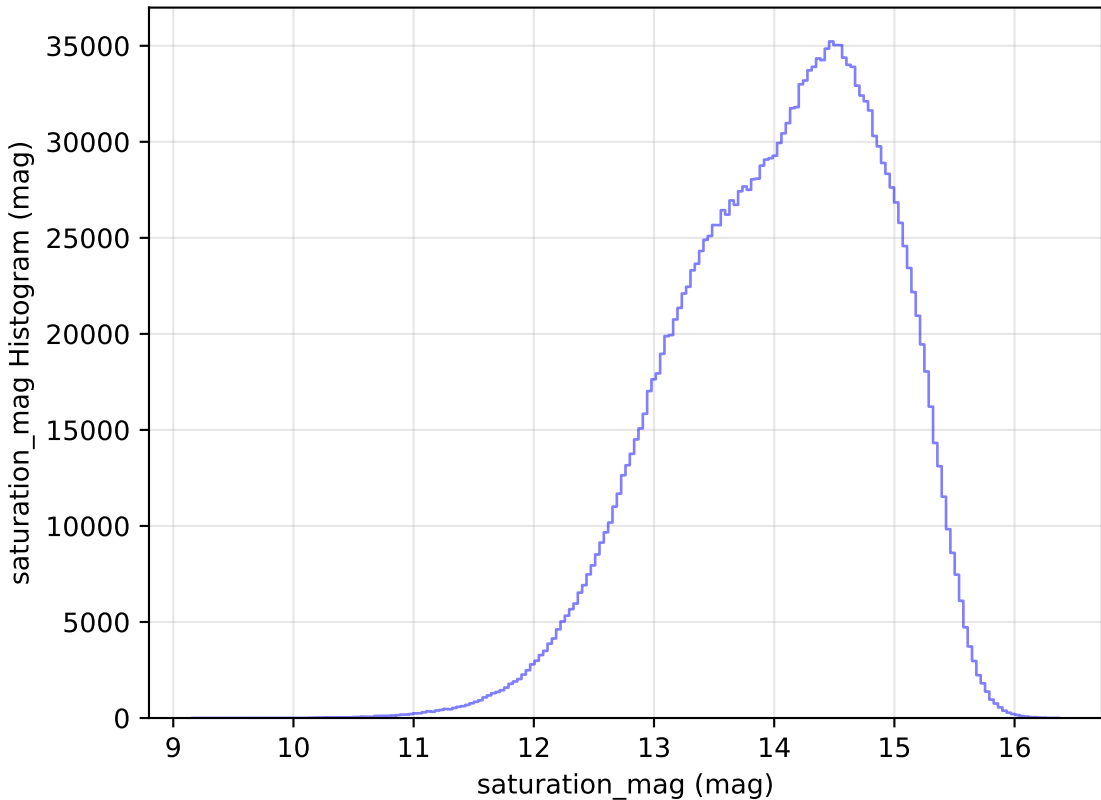
too_10_4v3.4_10yrs All sky all bands: saturation_mag Histogram
