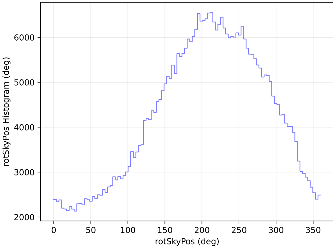
too_10_4v3.4_10yrs All sky z band: rotSkyPos Histogram
