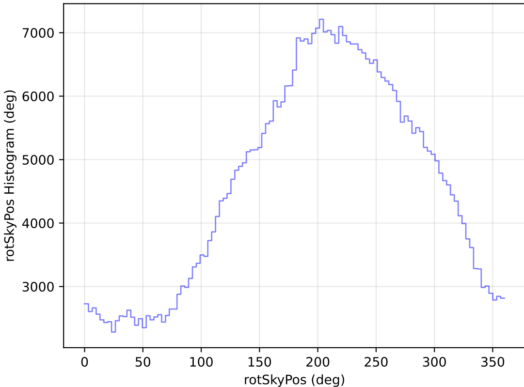
too_10_4v3.4_10yrs All sky i band: rotSkyPos Histogram
