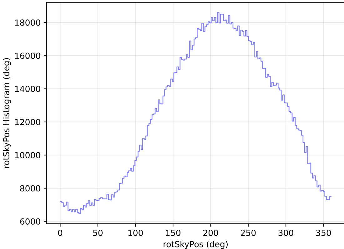
too_10_4v3.4_10yrs All sky all bands: rotSkyPos Histogram
