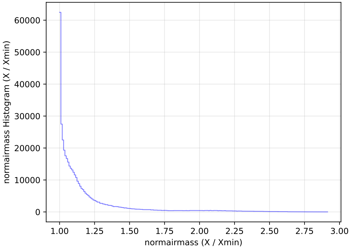
too_10_4v3.4_10yrs WFD z band: normairmass Histogram
