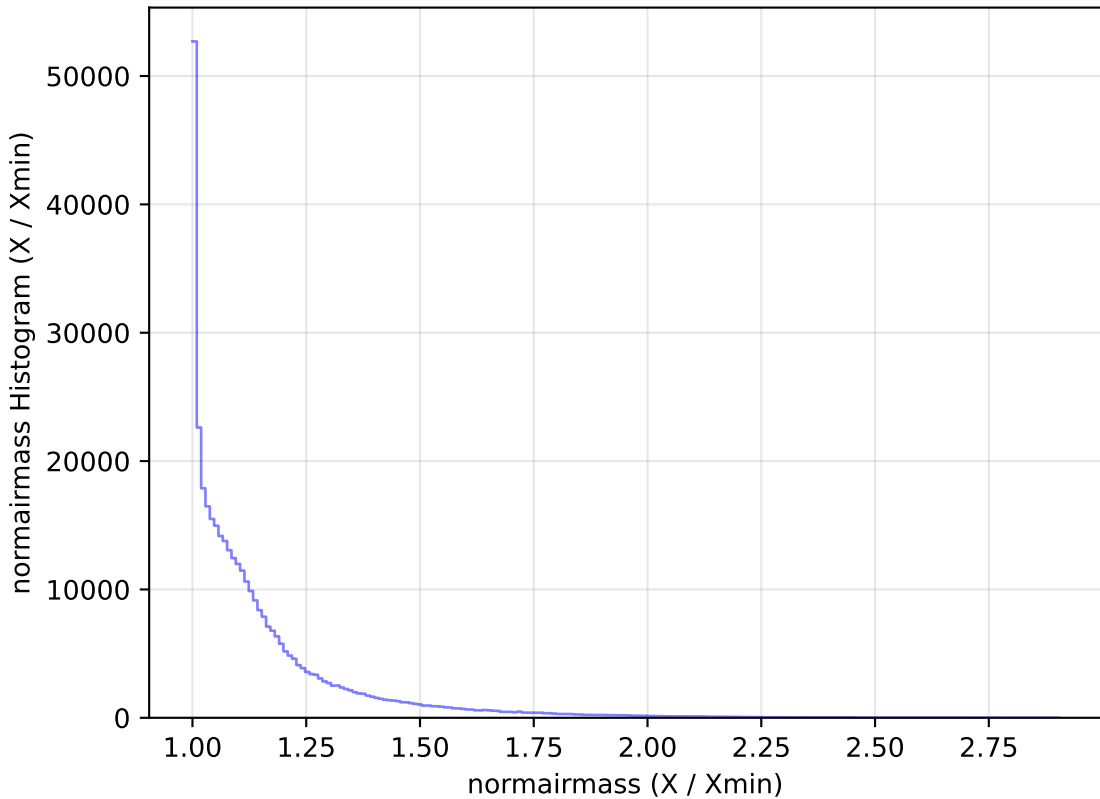
too_10_4v3.4_10yrs WFD y band: normairmass Histogram
