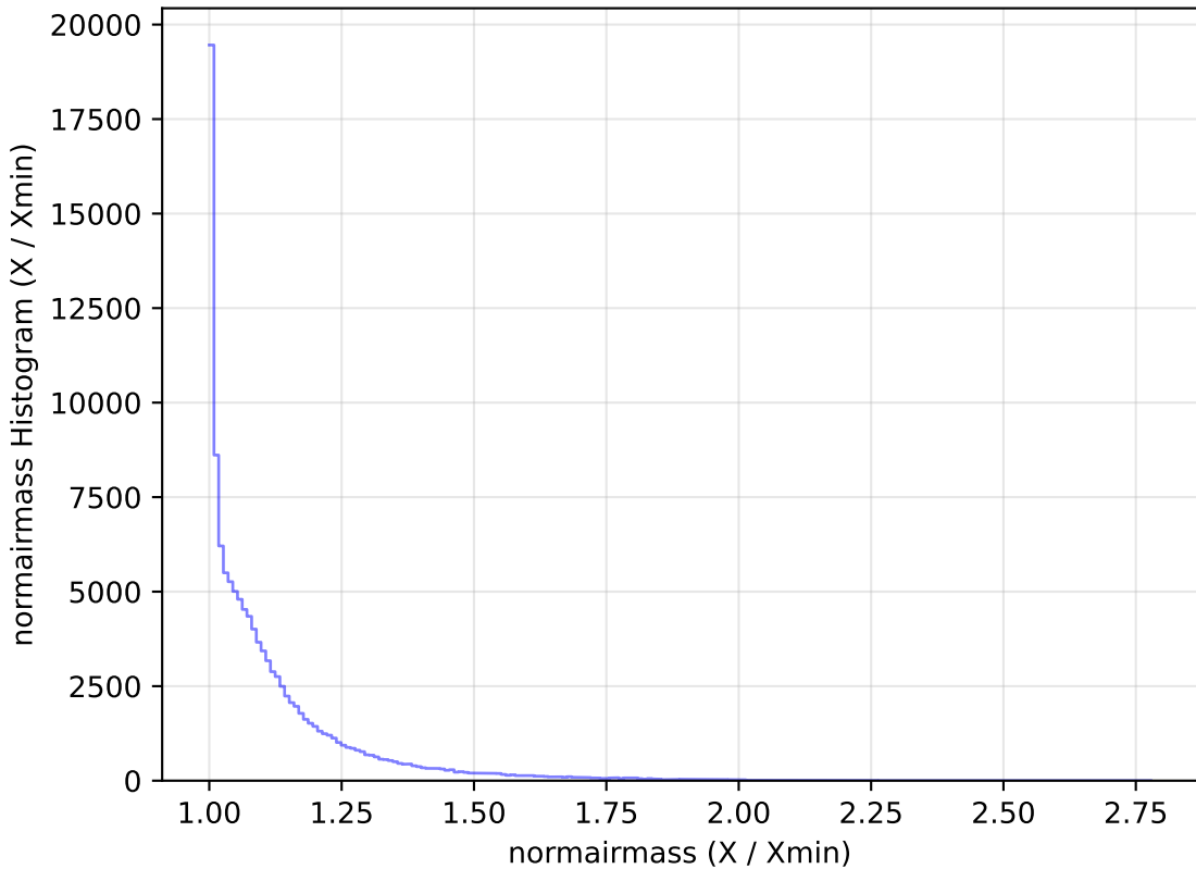
too_10_4v3.4_10yrs WFD u band: normairmass Histogram
