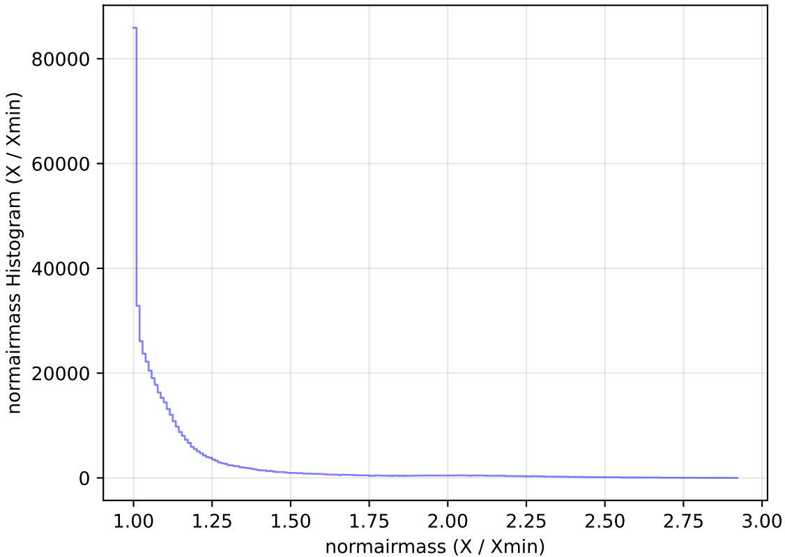
too_10_4v3.4_10yrs WFD i band: normairmass Histogram
