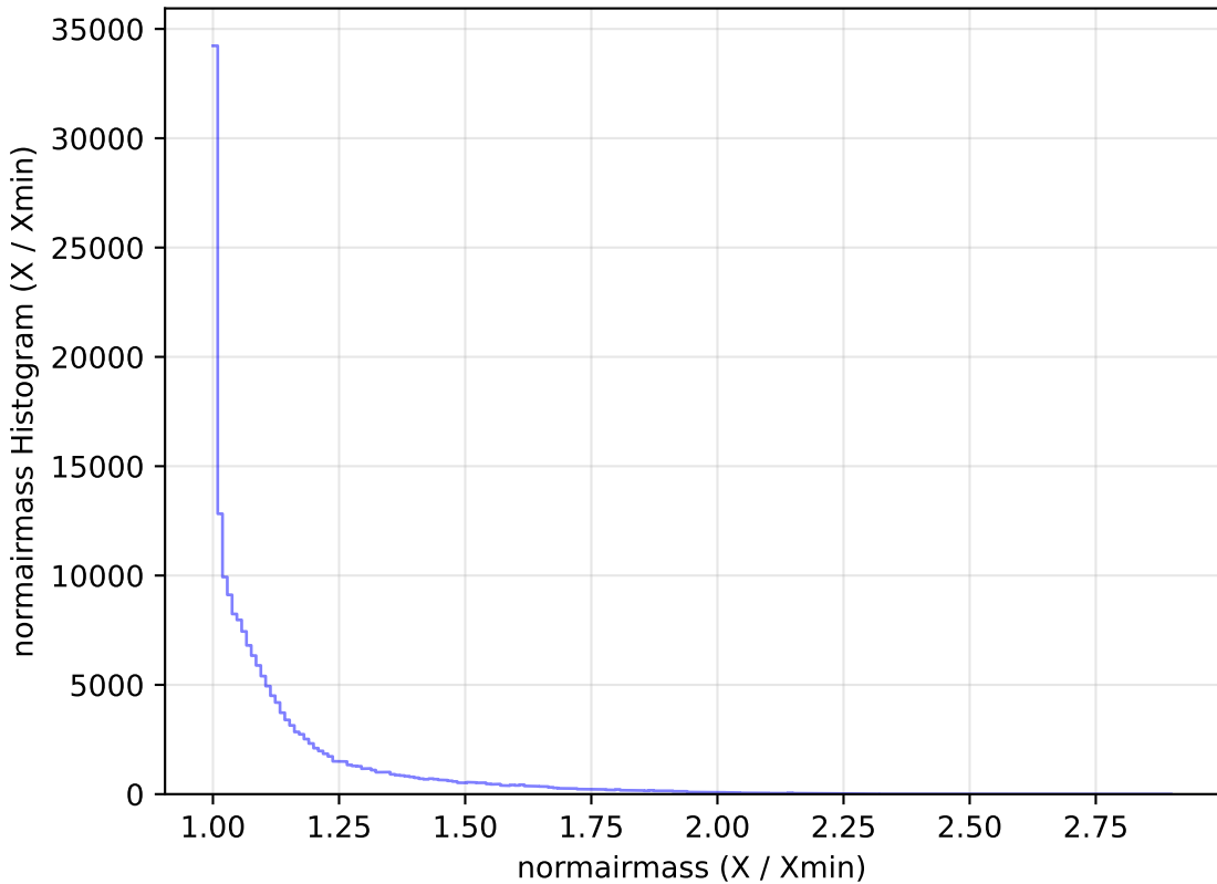
too_10_4v3.4_10yrs WFD g band: normairmass Histogram
