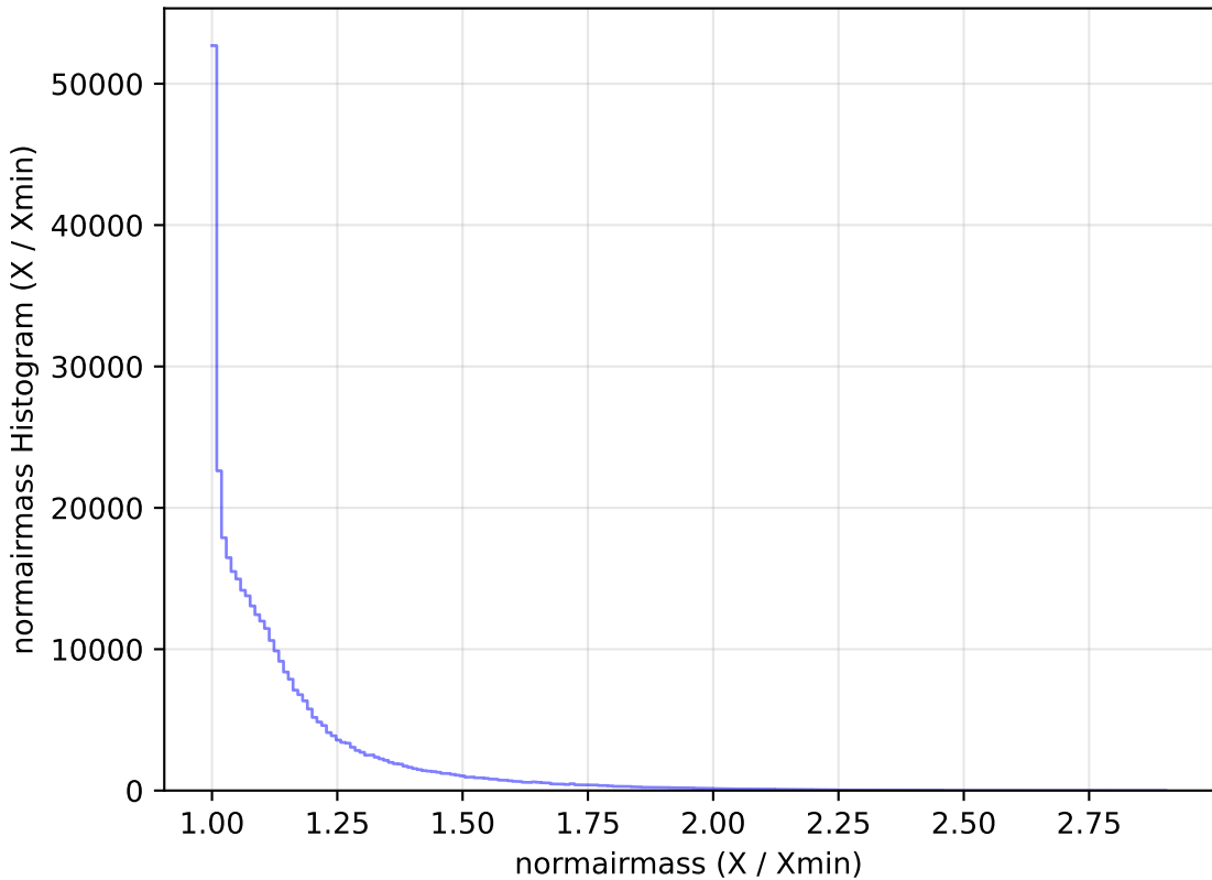
too_10_4v3.4_10yrs All sky y band: normairmass Histogram
