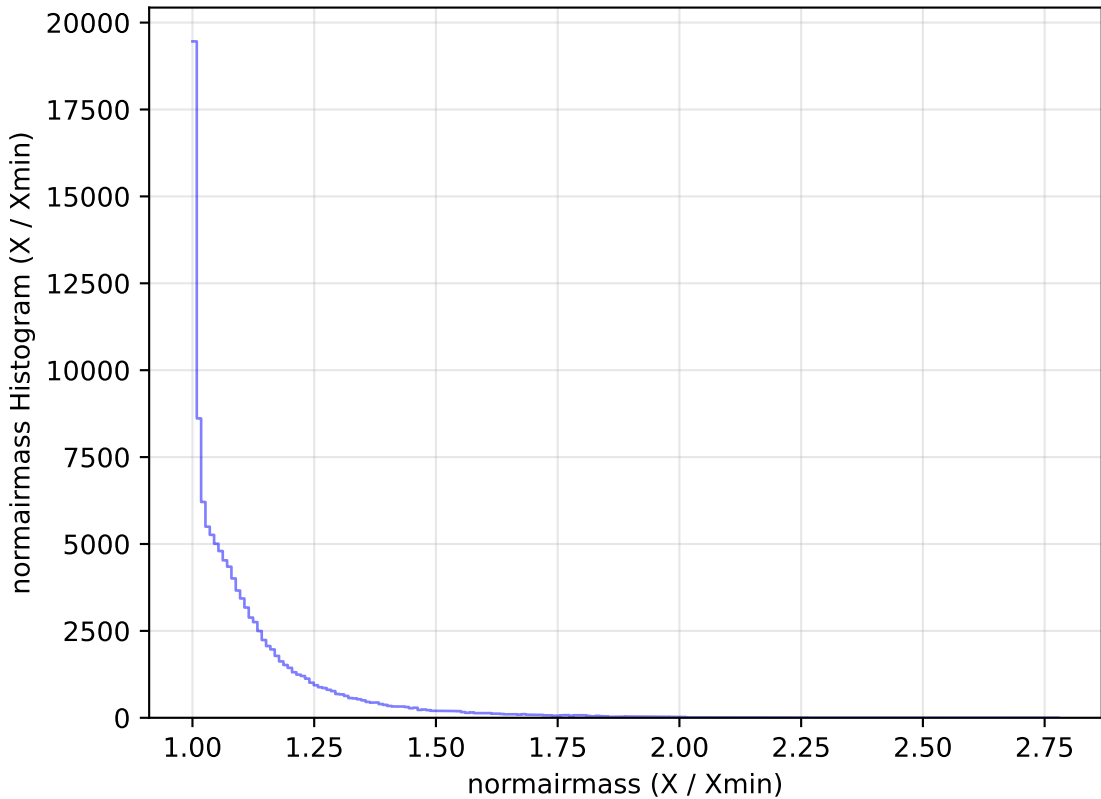
too_10_4v3.4_10yrs All sky u band: normairmass Histogram
