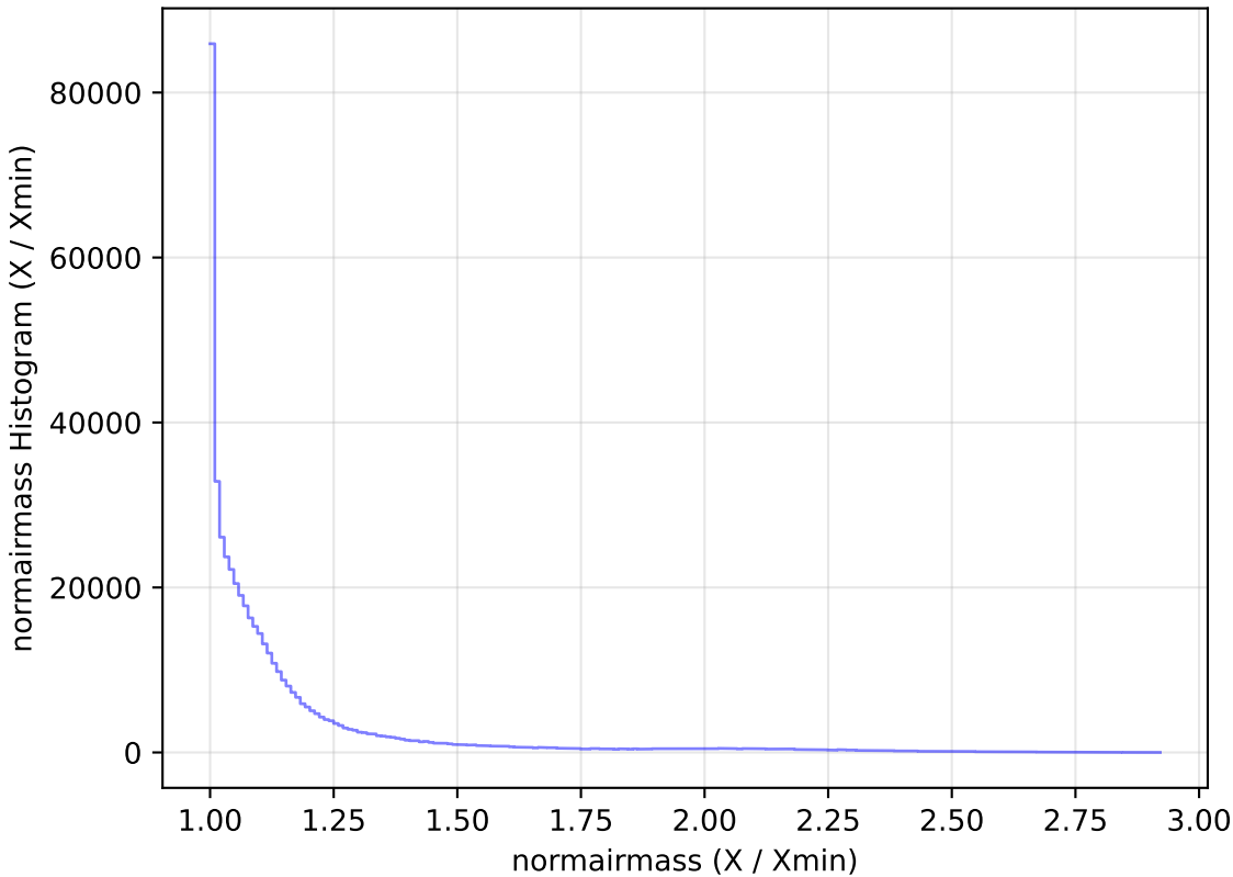
too_10_4v3.4_10yrs All sky i band: normairmass Histogram
