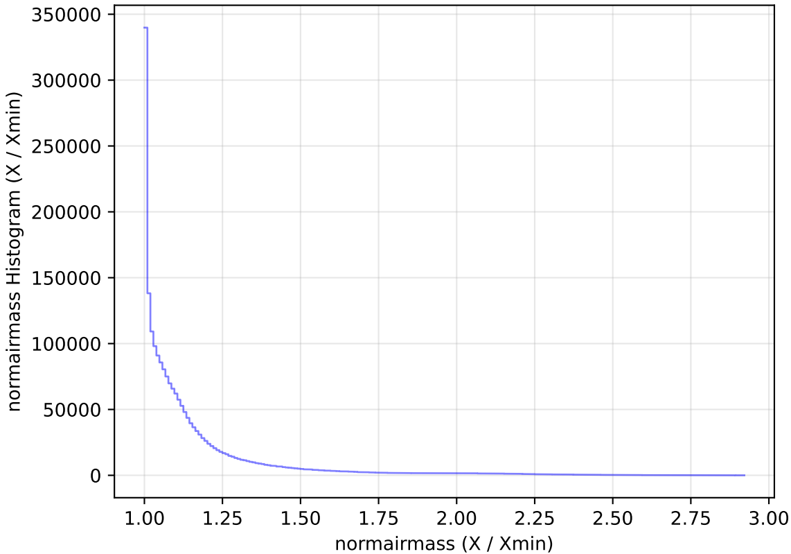
too_10_4v3.4_10yrs All sky all bands: normairmass Histogram
