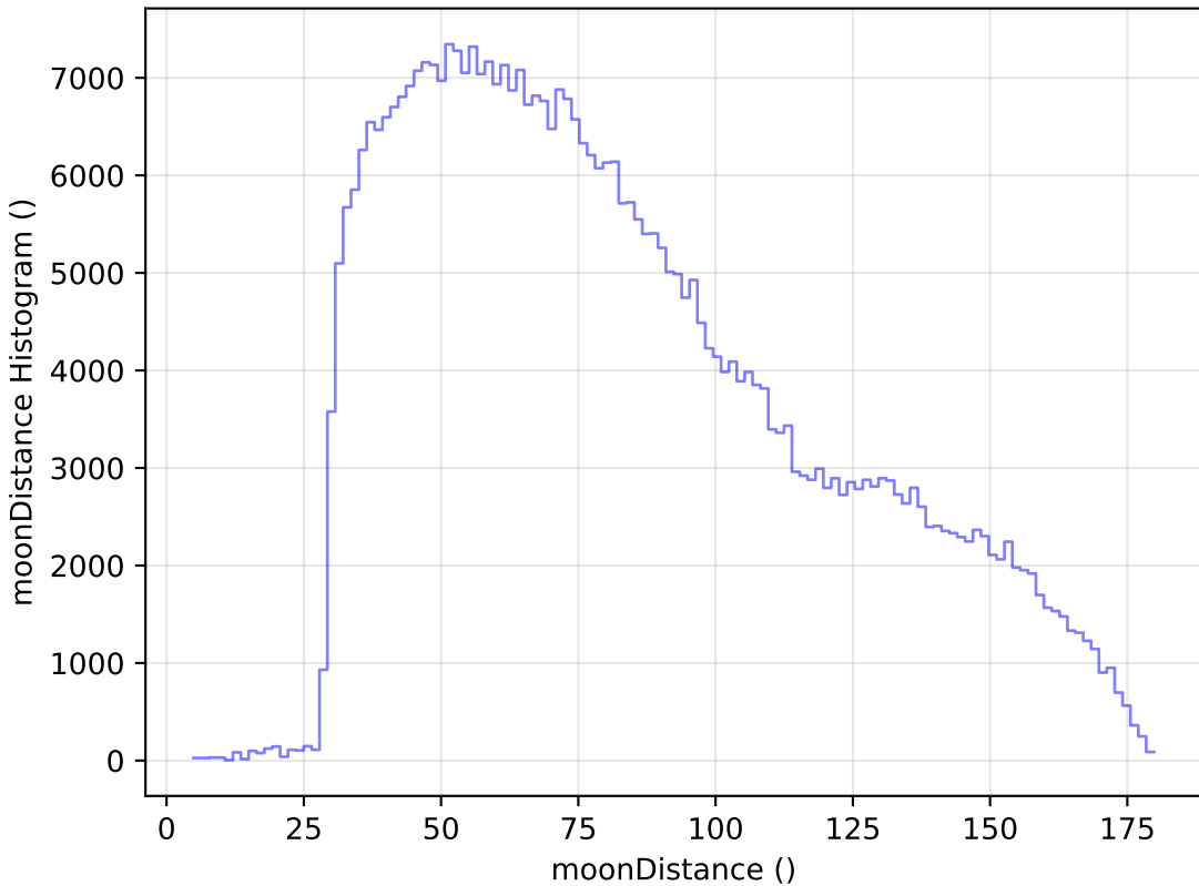
too_10_4v3.4_10yrs WFD z band: moonDistance Histogram
