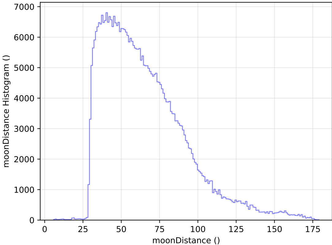
too_10_4v3.4_10yrs WFD y band: moonDistance Histogram
