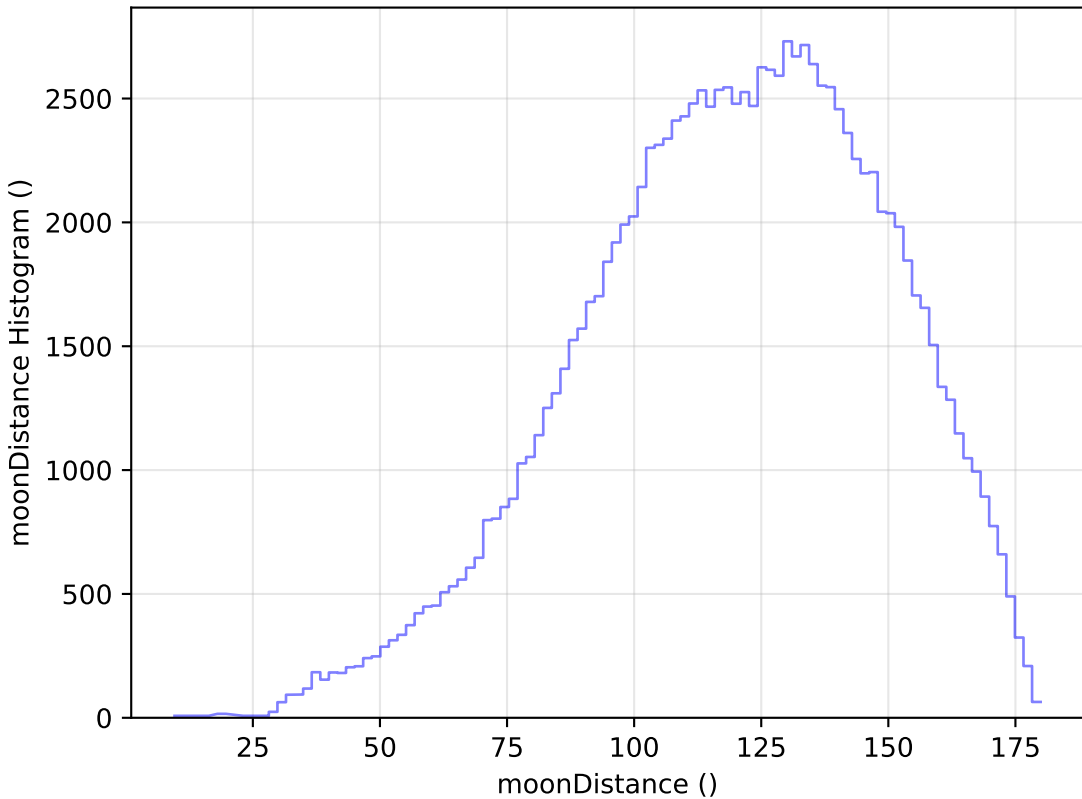
too_10_4v3.4_10yrs WFD u band: moonDistance Histogram
