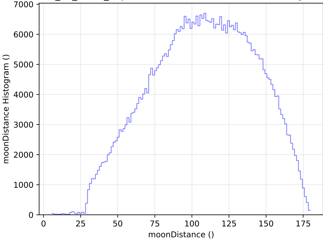
too_10_4v3.4_10yrs WFD r band: moonDistance Histogram
