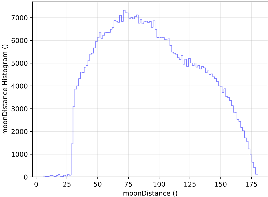
too_10_4v3.4_10yrs WFD i band: moonDistance Histogram
