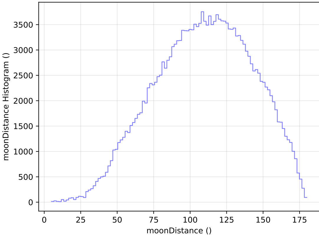
too_10_4v3.4_10yrs WFD g band: moonDistance Histogram
