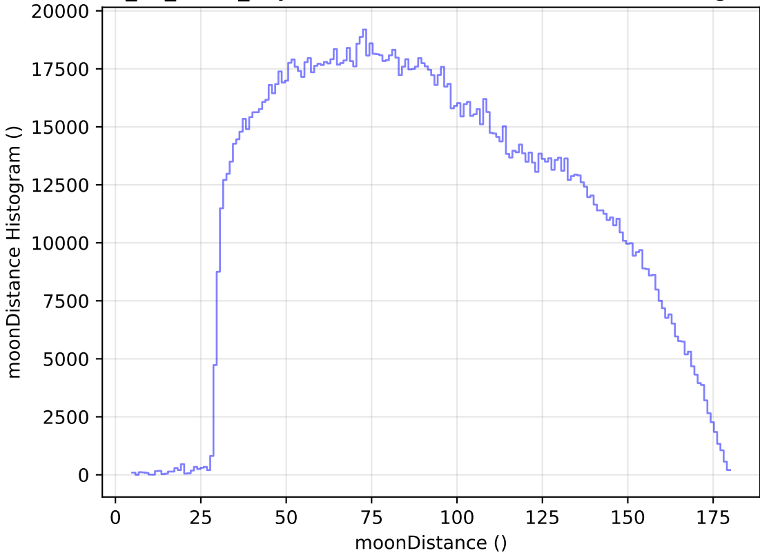
too_10_4v3.4_10yrs WFD all bands: moonDistance Histogram
