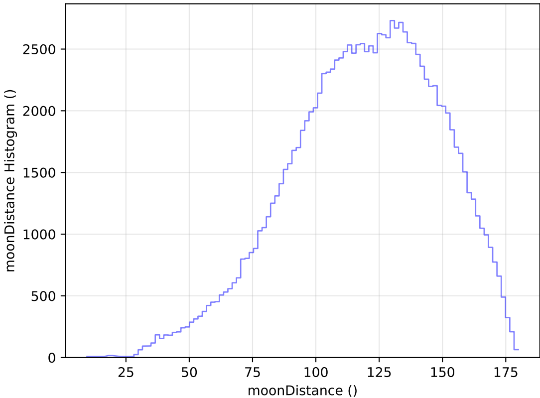
too_10_4v3.4_10yrs All sky u band: moonDistance Histogram
