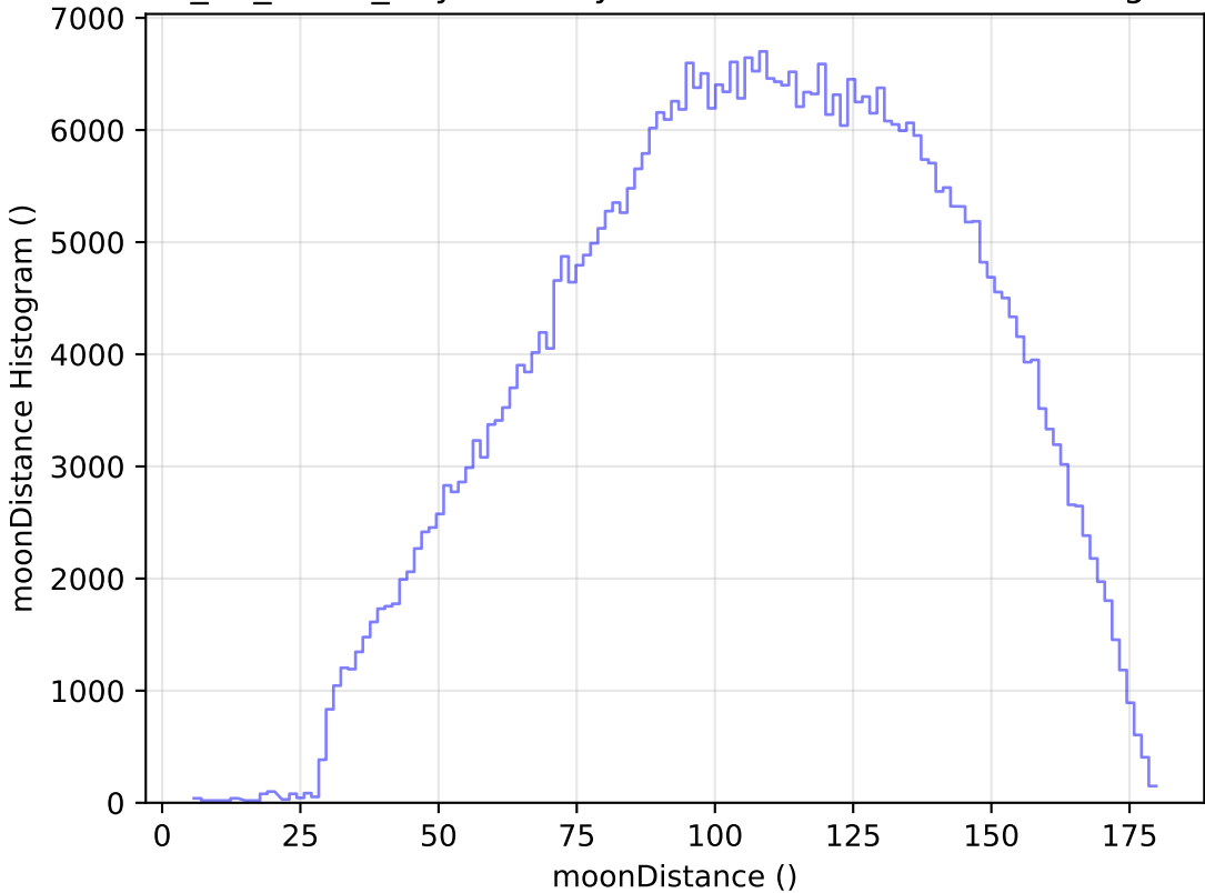
too_10_4v3.4_10yrs All sky r band: moonDistance Histogram
