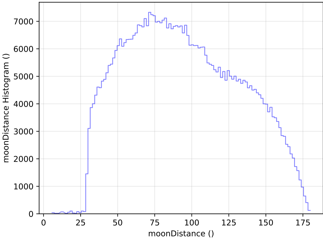
too_10_4v3.4_10yrs All sky i band: moonDistance Histogram
