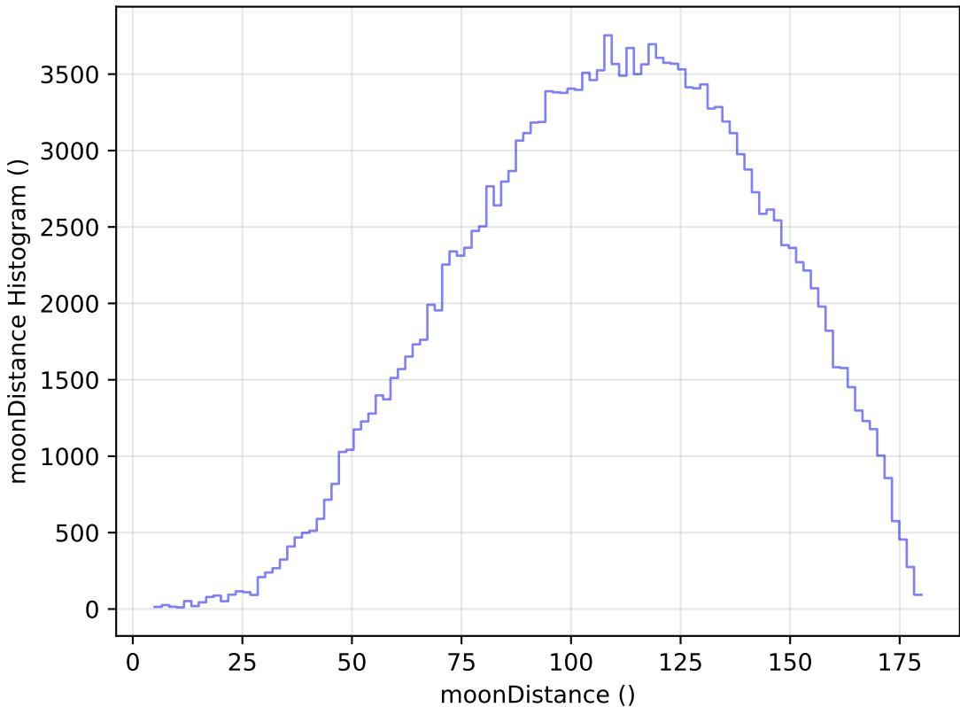
too_10_4v3.4_10yrs All sky g band: moonDistance Histogram
