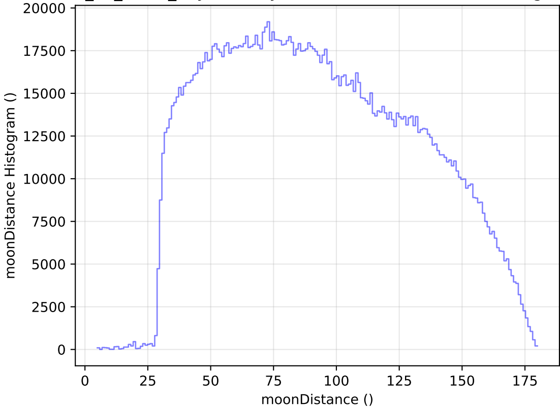
too_10_4v3.4_10yrs All sky all bands: moonDistance Histogram
