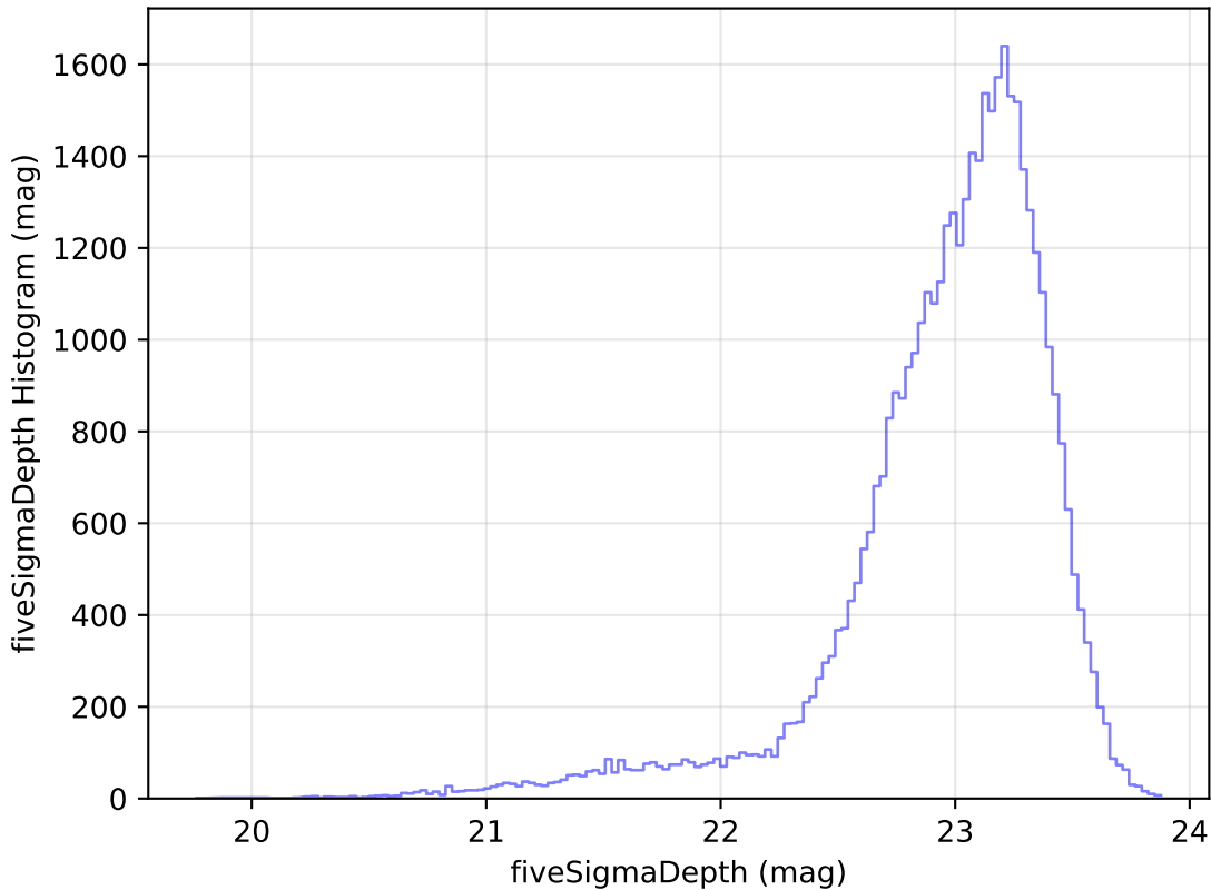
too_10_4v3.4_10yrs Yr 1 z band: fiveSigmaDepth Histogram
