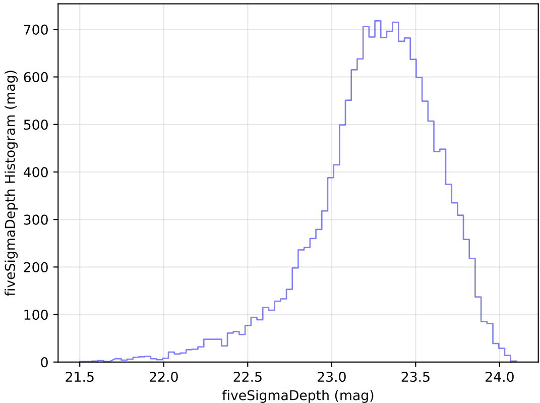
too_10_4v3.4_10yrs Yr 1 u band: fiveSigmaDepth Histogram
