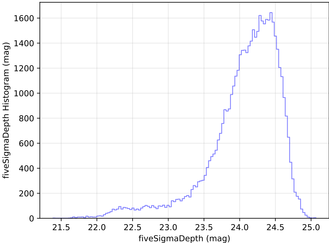
too_10_4v3.4_10yrs Yr 1 r band: fiveSigmaDepth Histogram
