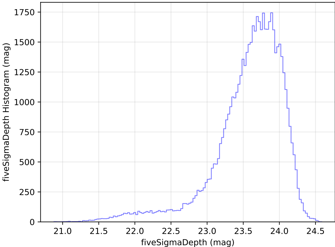
too_10_4v3.4_10yrs Yr 1 i band: fiveSigmaDepth Histogram
