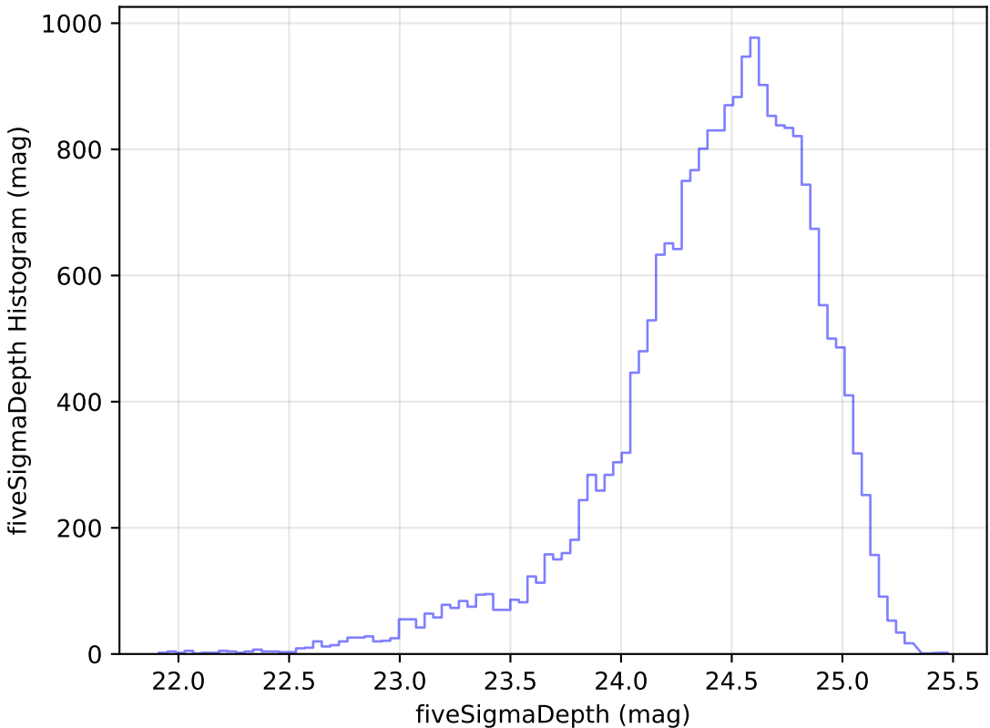
too_10_4v3.4_10yrs Yr 1 g band: fiveSigmaDepth Histogram
