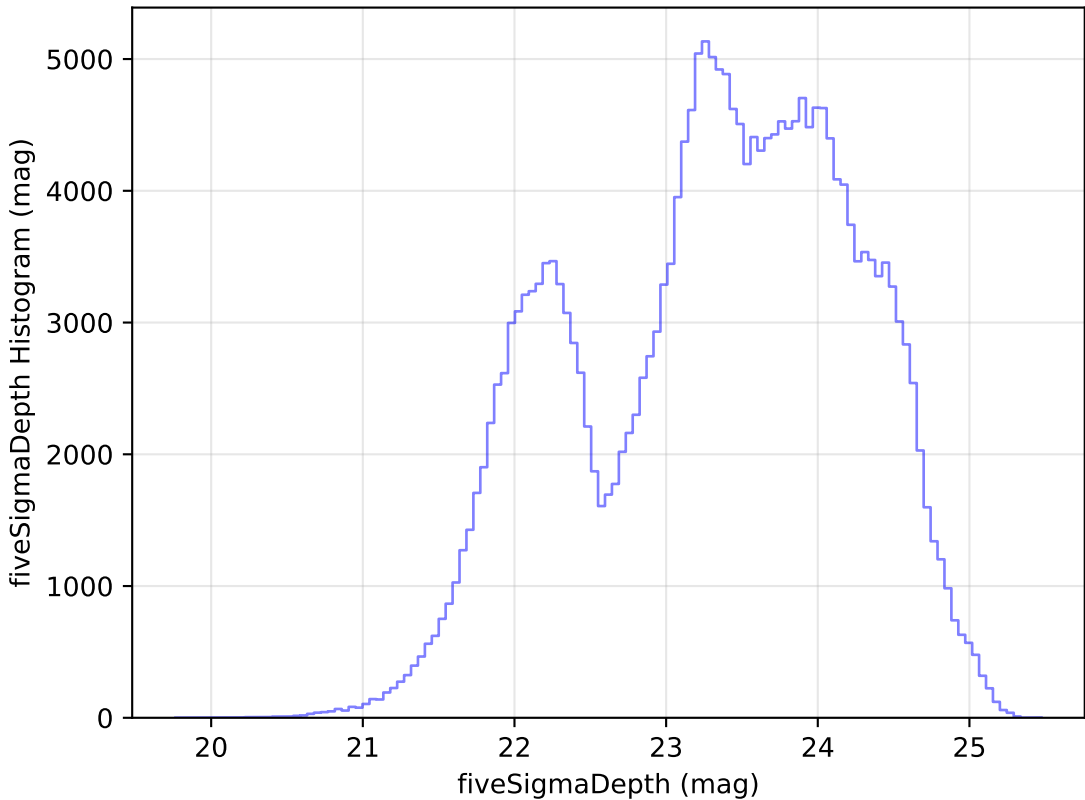
too_10_4v3.4_10yrs Yr 1 all bands: fiveSigmaDepth Histogram
