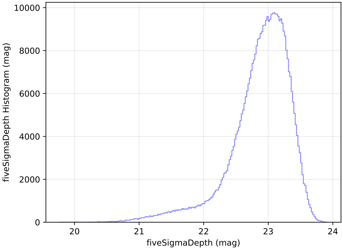
too_10_4v3.4_10yrs WFD z band: fiveSigmaDepth Histogram
