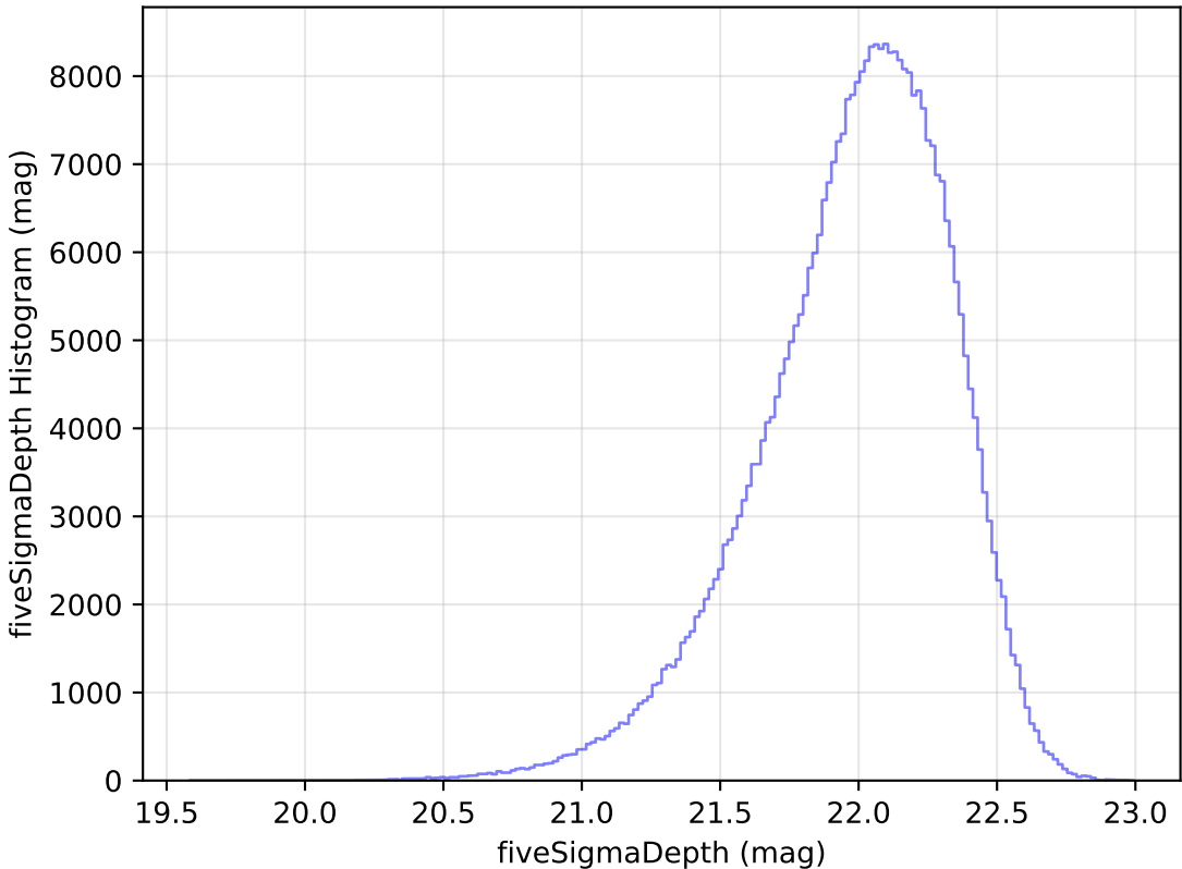
too_10_4v3.4_10yrs WFD y band: fiveSigmaDepth Histogram
