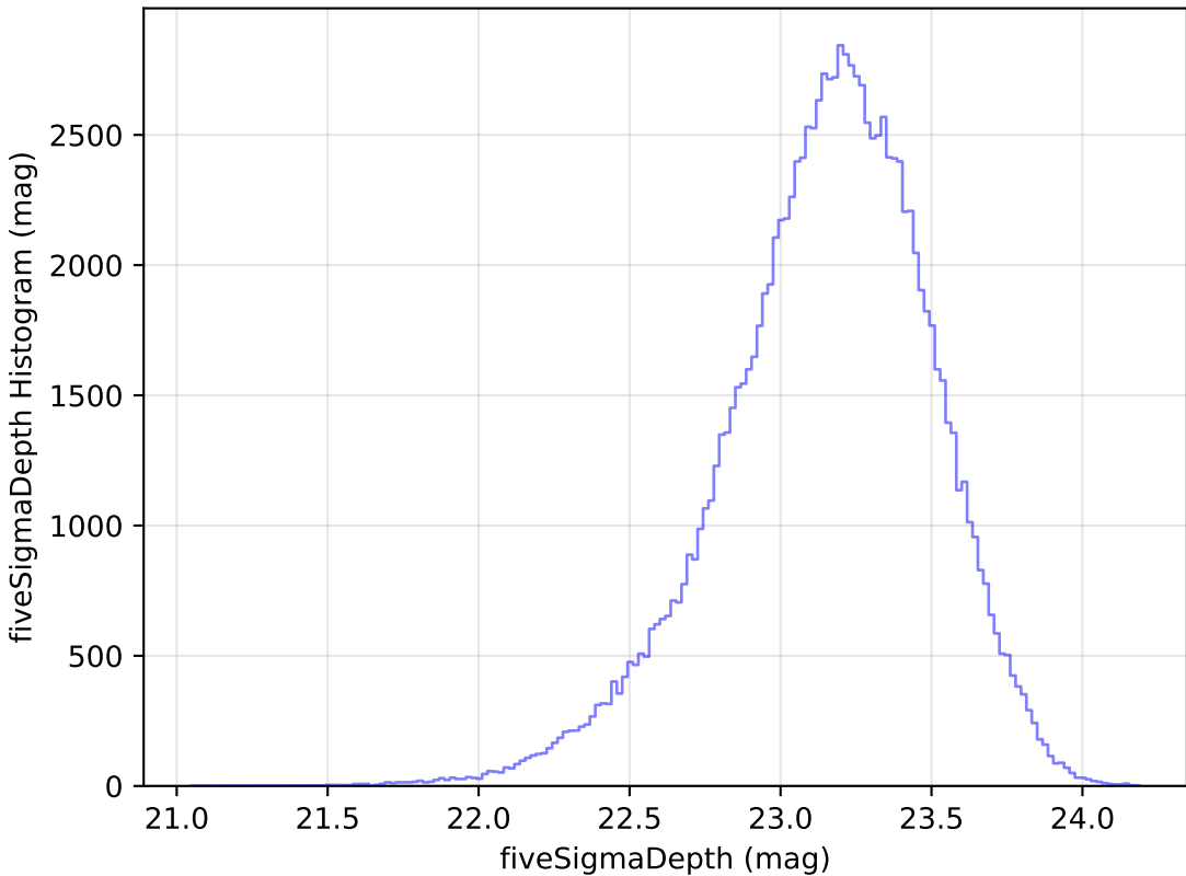
too_10_4v3.4_10yrs WFD u band: fiveSigmaDepth Histogram
