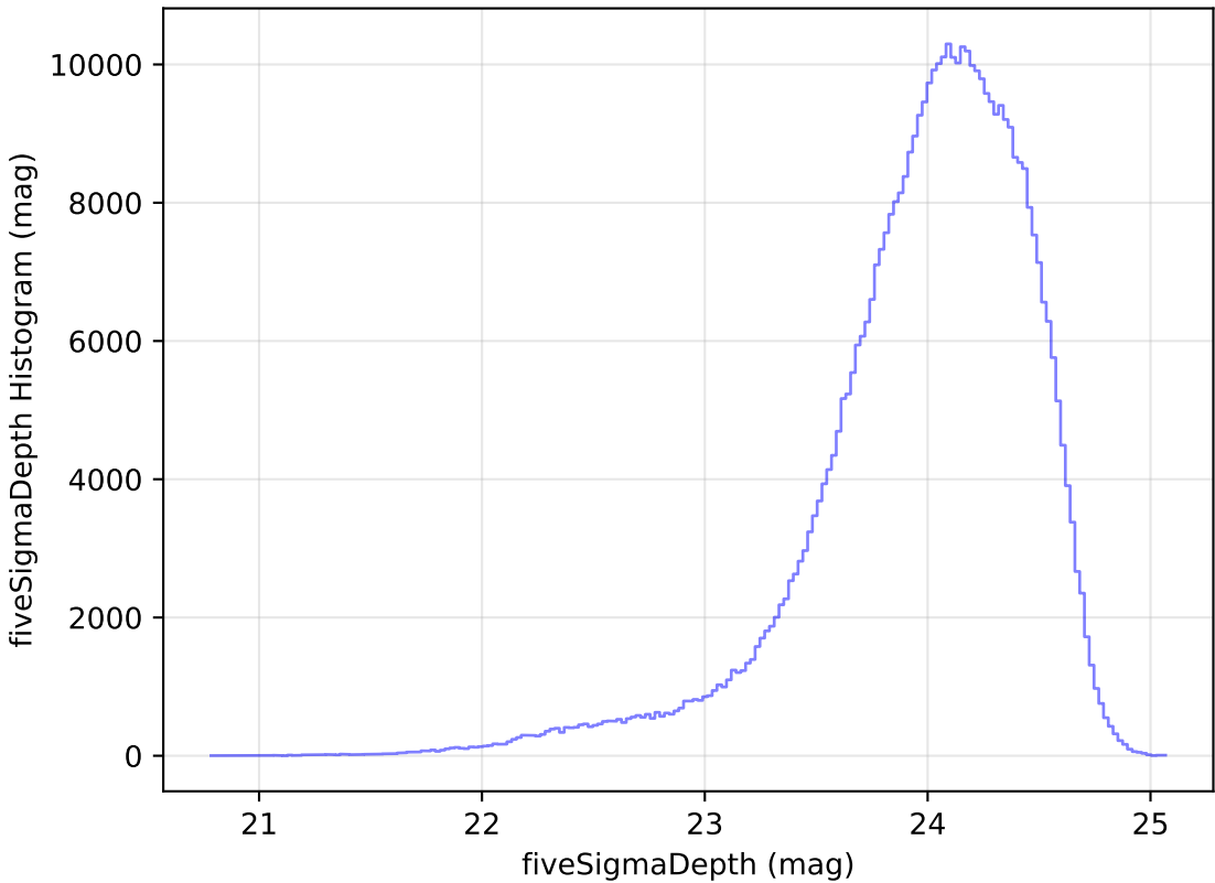
too_10_4v3.4_10yrs WFD r band: fiveSigmaDepth Histogram
