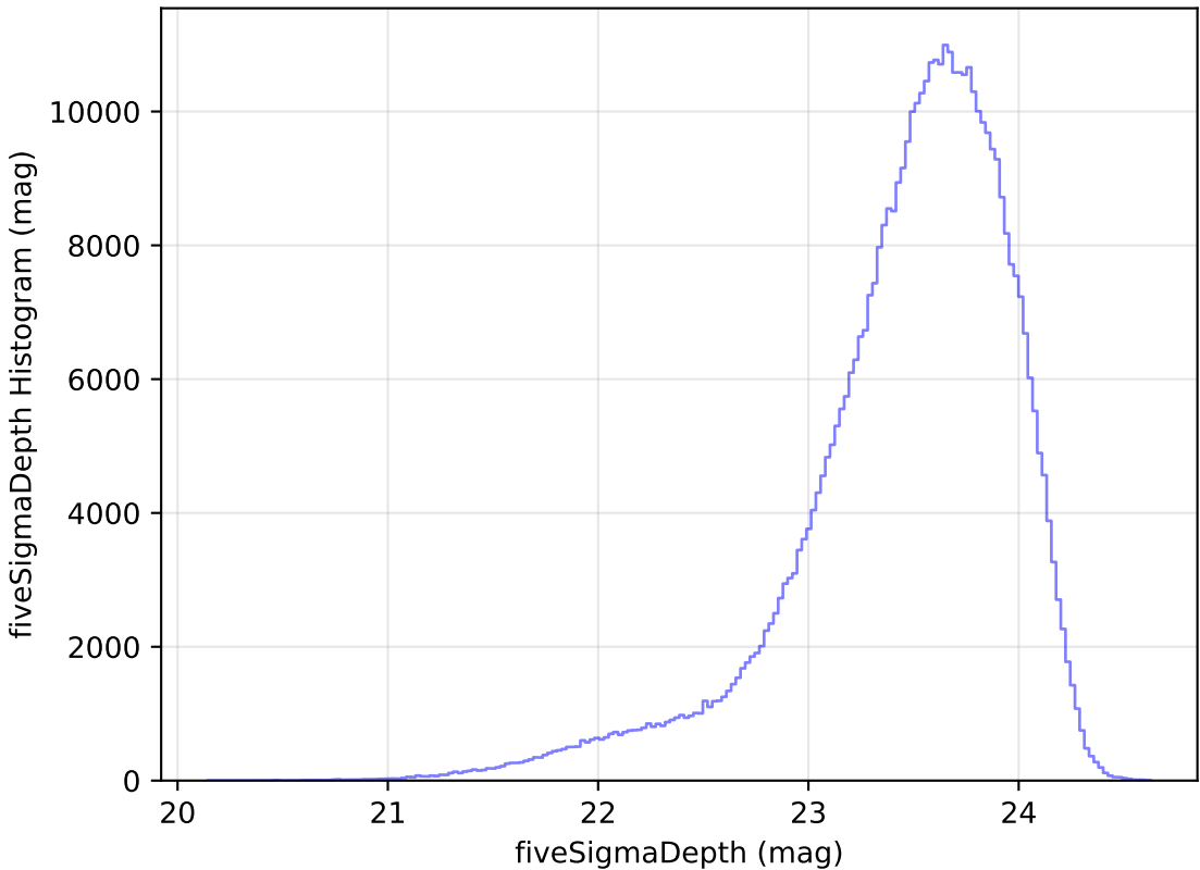
too_10_4v3.4_10yrs WFD i band: fiveSigmaDepth Histogram
