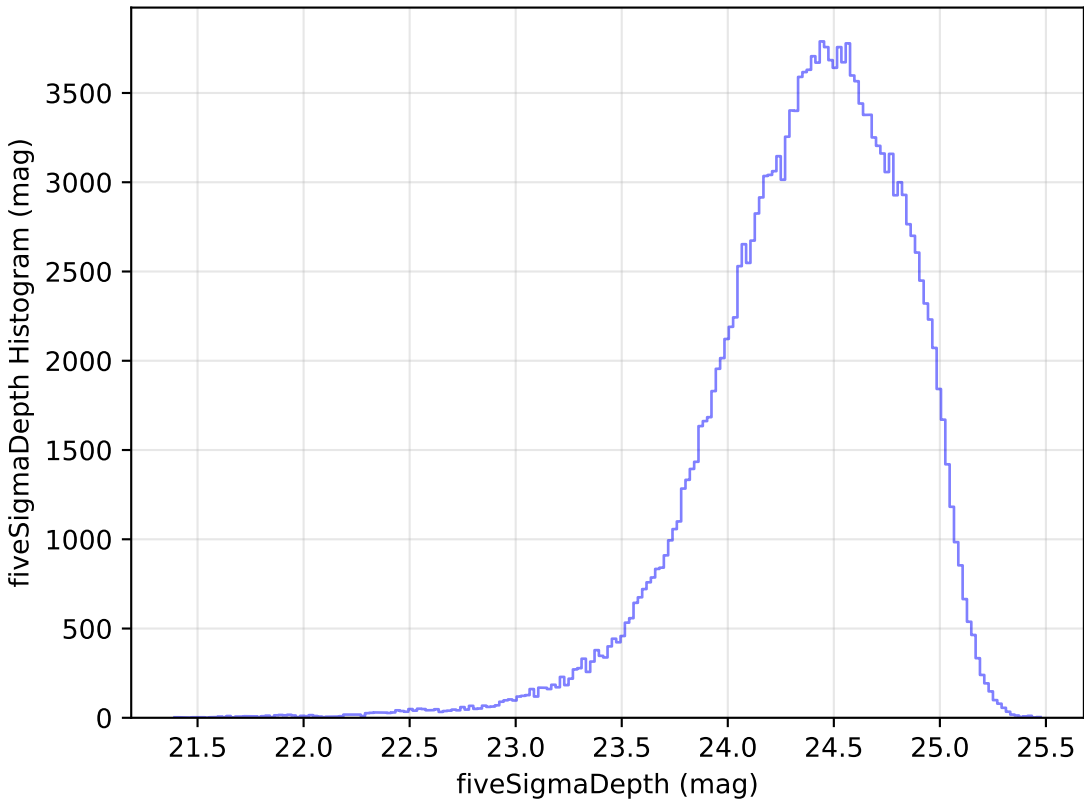
too_10_4v3.4_10yrs WFD g band: fiveSigmaDepth Histogram
