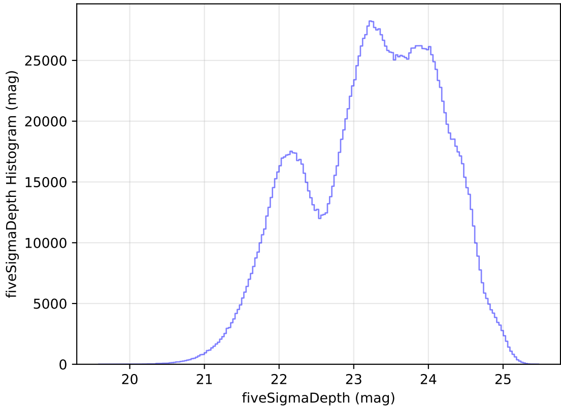
too_10_4v3.4_10yrs WFD all bands: fiveSigmaDepth Histogram
