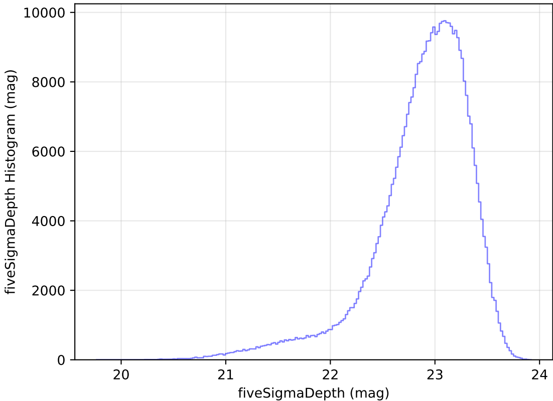
too_10_4v3.4_10yrs All sky z band: fiveSigmaDepth Histogram
