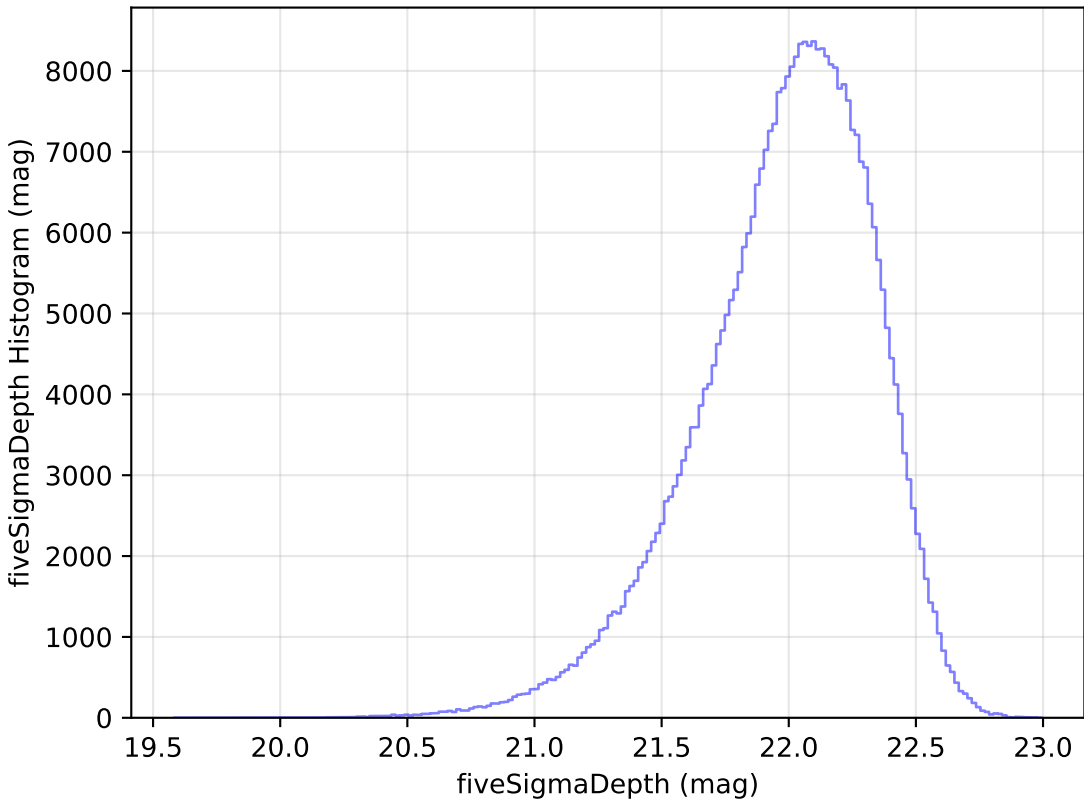
too_10_4v3.4_10yrs All sky y band: fiveSigmaDepth Histogram
