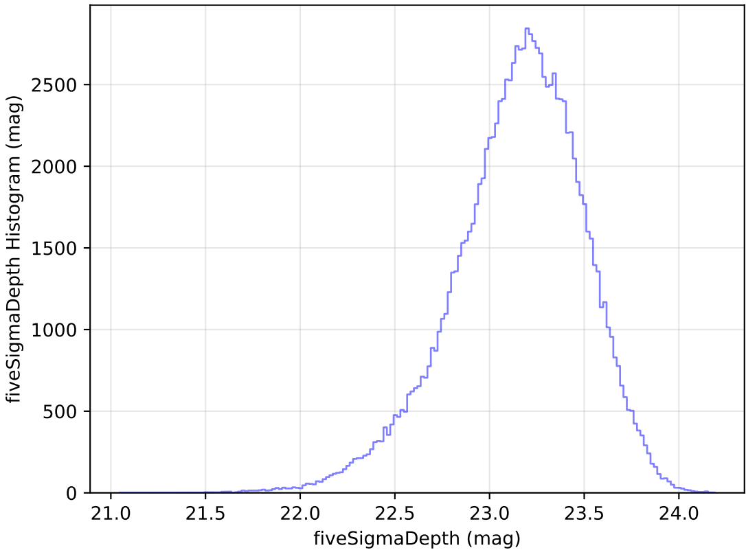
too_10_4v3.4_10yrs All sky u band: fiveSigmaDepth Histogram
