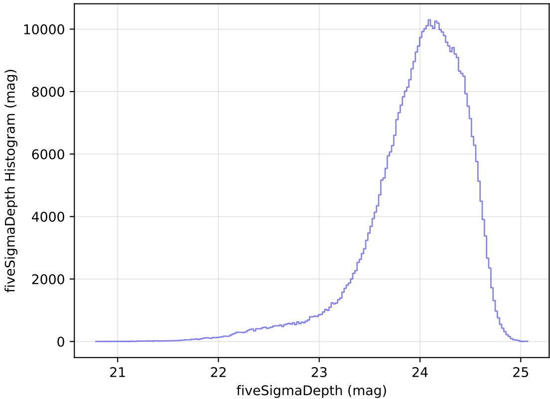
too_10_4v3.4_10yrs All sky r band: fiveSigmaDepth Histogram
