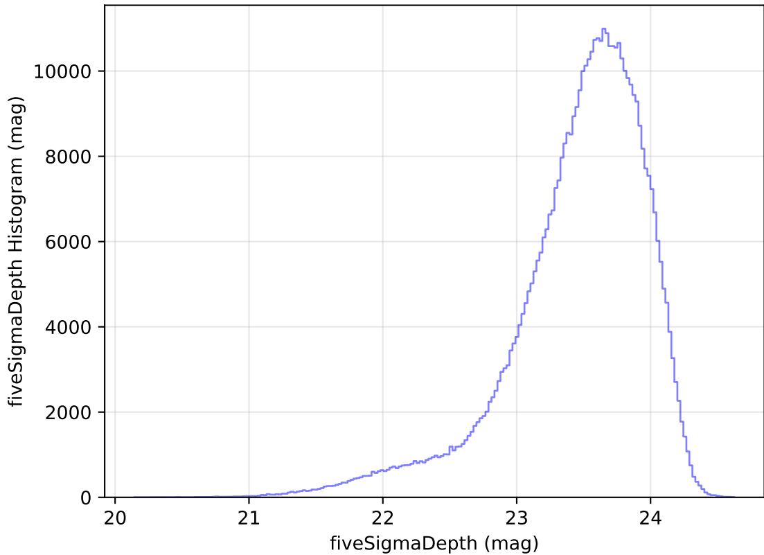
too_10_4v3.4_10yrs All sky i band: fiveSigmaDepth Histogram
