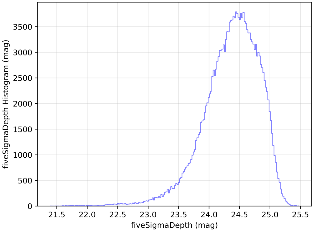
too_10_4v3.4_10yrs All sky g band: fiveSigmaDepth Histogram
