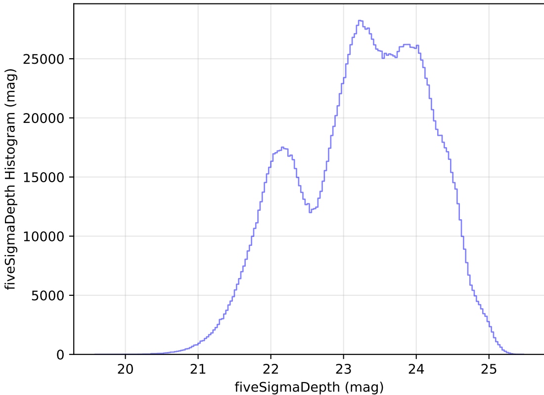
too_10_4v3.4_10yrs All sky all bands: fiveSigmaDepth Histogram
