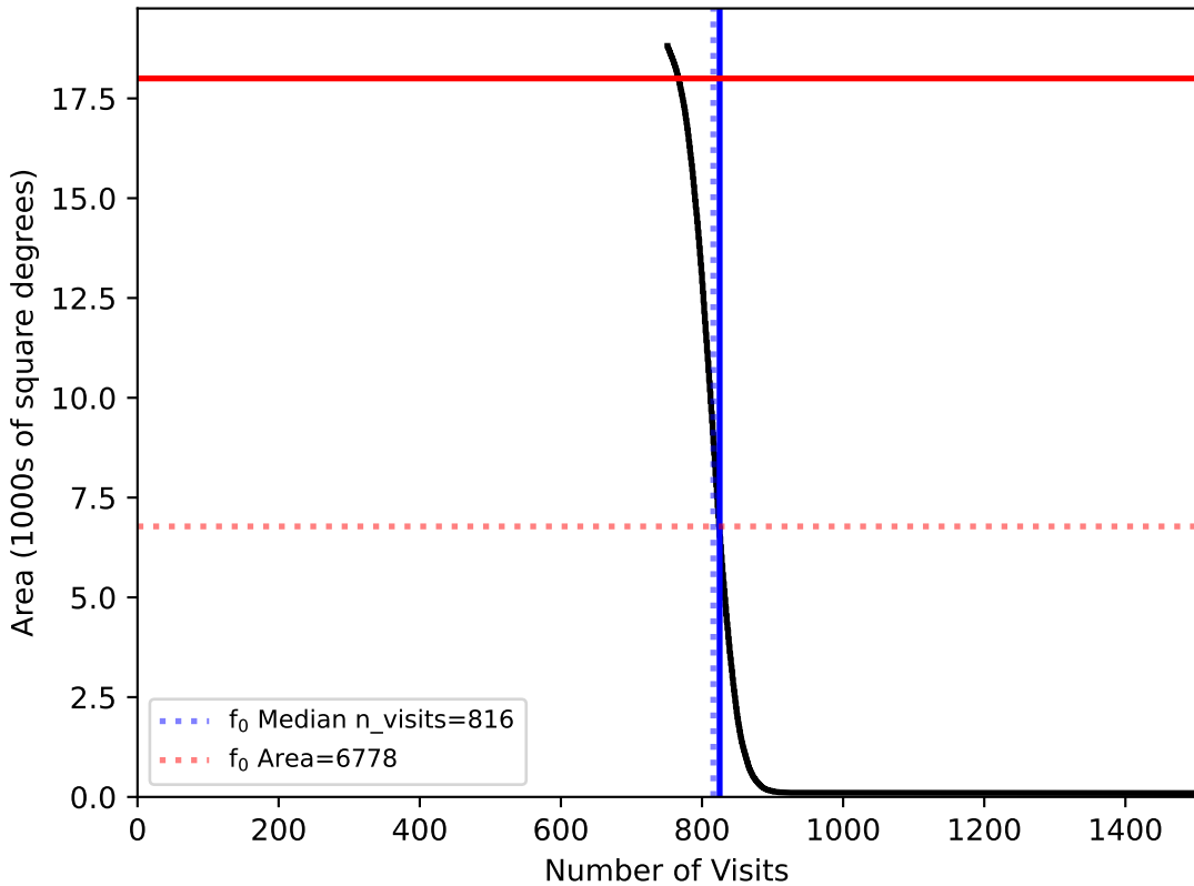
too_10_4v3.4_10yrs WFD: f0
