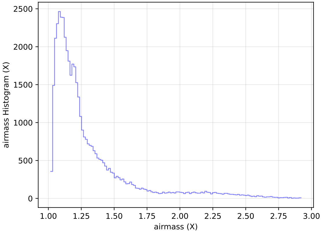
too_10_4v3.4_10yrs Yr 1 z band: airmass Histogram
